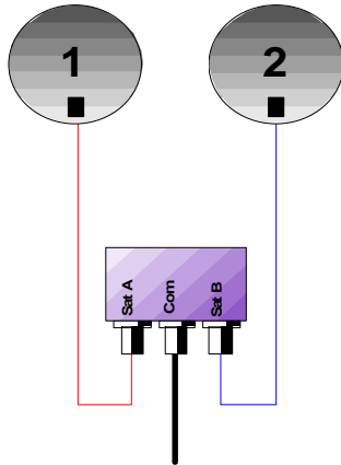
Commutatore per 2 satelliti *22 kHz *ToneBurst (MiniDiSEqC) *DiSEqC Committed o Uncommitted
