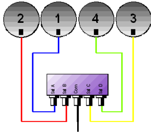
Commutatore per 4 satelliti * DiSEqC Committed o Uncommitted
