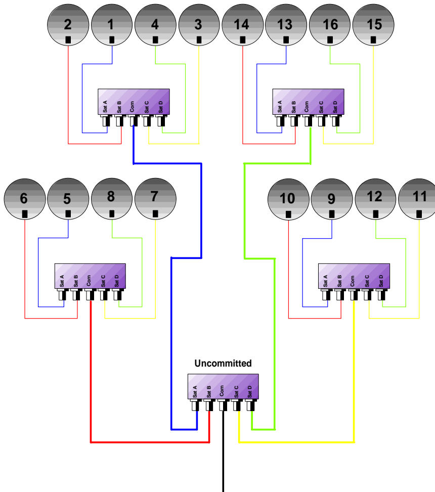
Commutatore per 16 satelliti * DiSEqC Committed + Uncommitted
